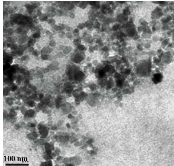
Fig.1. Large area TEM image of \text{Fe}_2\text{O}_3 nanoparticles.
